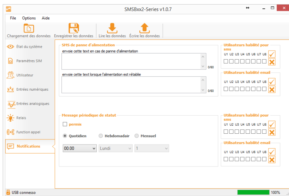
Figure 1: Notification
